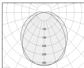
Lysfordeling for PL5000
